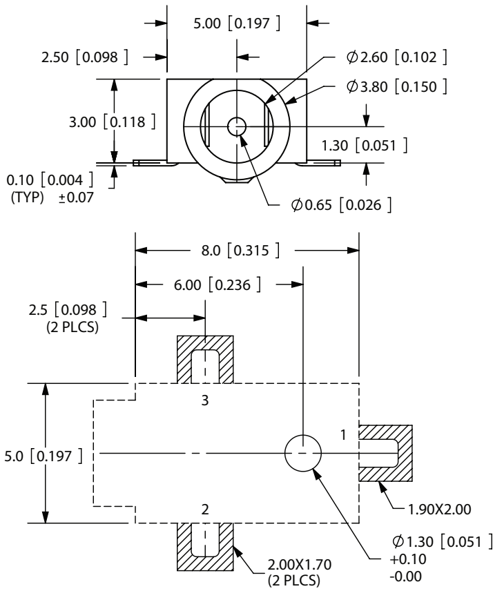
PCB LAYOUT TOP VIEW
