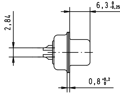
Solder bucket for AWG 20
